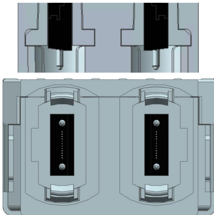
Figure 7.3.1 Dual MPO12 APC interface
