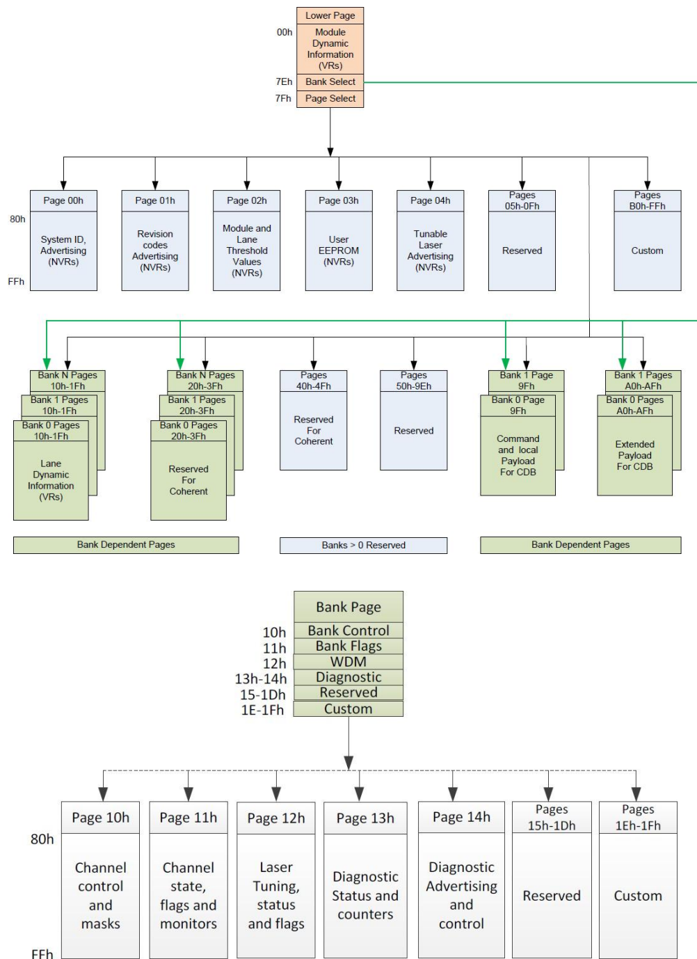
Figure 5.1 CMIS Module Memory Map
