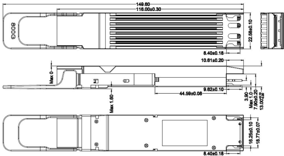
Figure 7.1 Package dimensions
