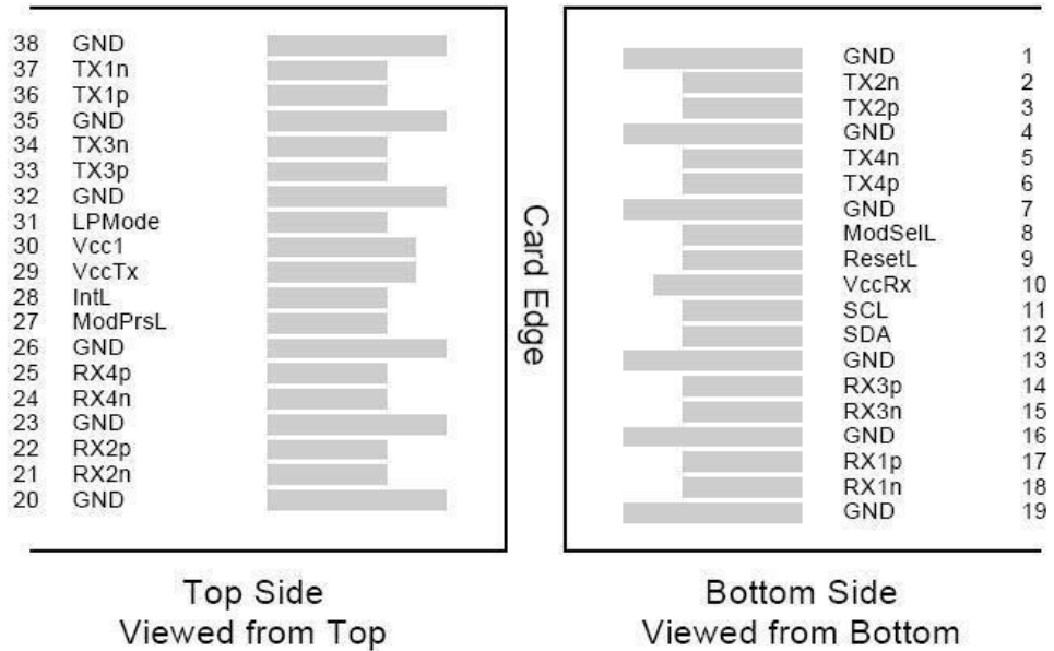
Figure 2: Pin Definitions
